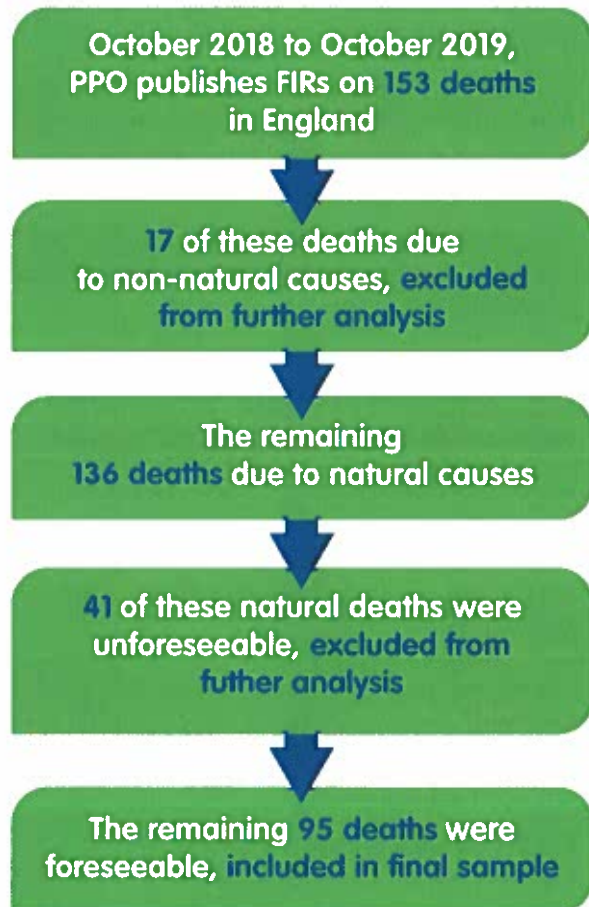
Figure 4: Diagram demonstrating how the final sample of PPO FIRs was chosen
